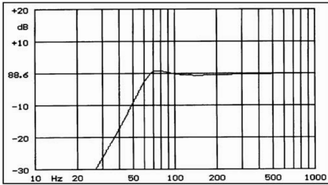
Frequenzgang- Bass: Computer- Simulation
